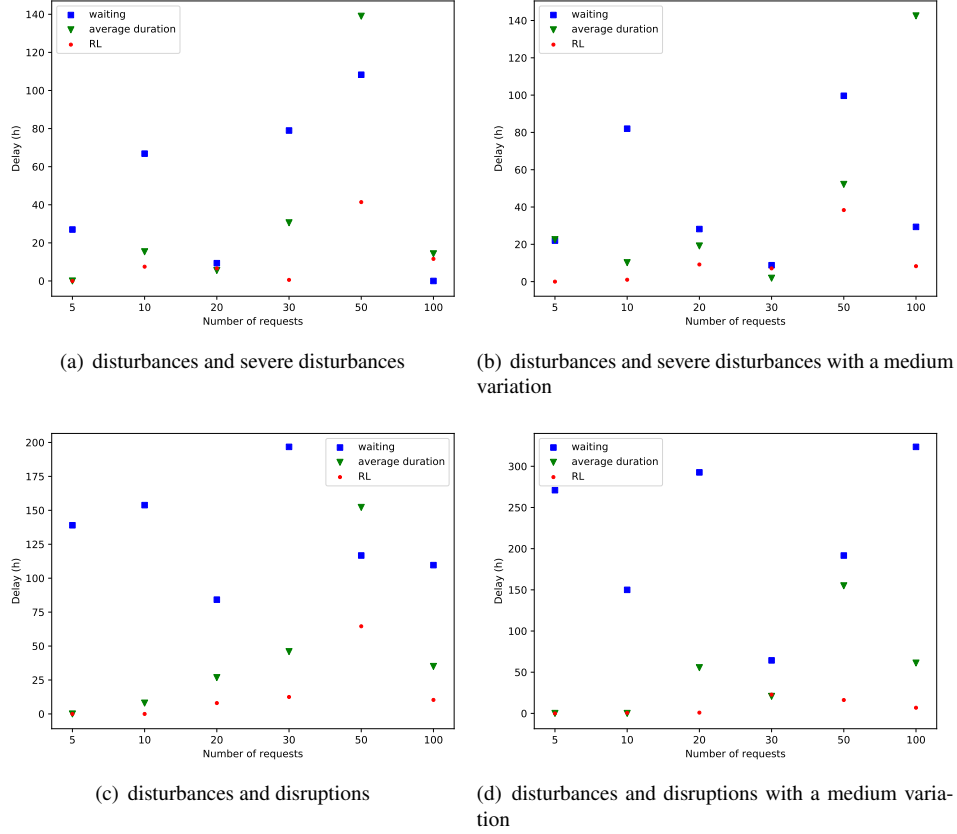
Figure 4.14: Total delay over all requests under different types of events occurring at different terminals.
