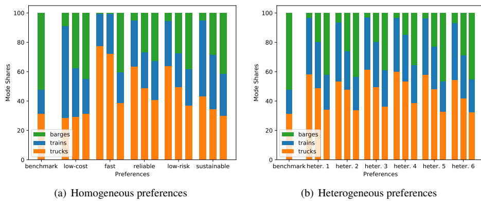
Figure 6.7: Mode shares under homogeneous and heterogeneous preferences. The three bars from left to right of each instance are results under hard constraints, fuzzy constraints, and the satisfaction objective, respectively.
