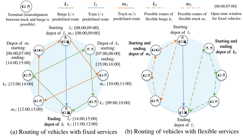
Figure 3.1: Routing of vehicles with fixed and flexible services in synchronodal transport.
